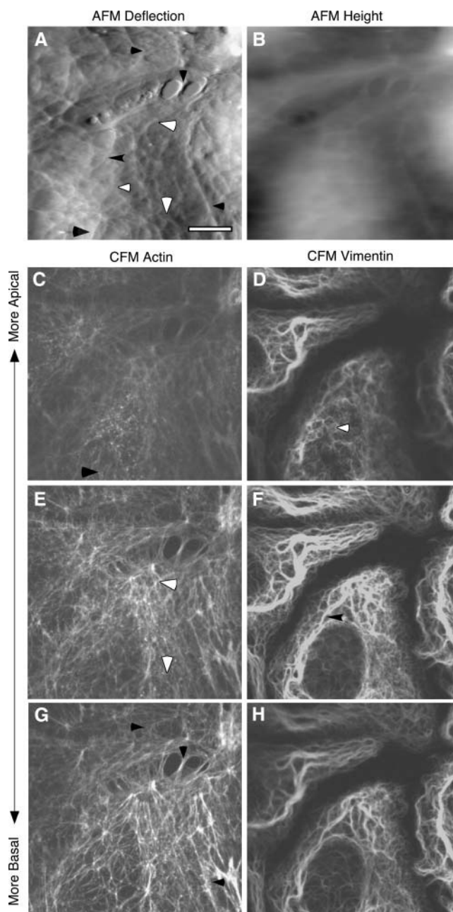
FIGURE 6 Correlated AFM and CFM of cells double stained for actin and vimentin. AFM image on living BPAECs was collected and the cells were immediately fixed and processed for immunofluorescence. (A) The deflection image shows details of the mesh-like cortical organization, whereas (B) the height image better reflects the overall cell shape. Confocal planes of cells stained for actin using Alexa-phalloidin (C, E, and G) and vimentin using Cy3-anti-vimentin antibody (D, F, and H). Correlated features are marked with arrowheads. Scale bar is 10 \mu\text{m} . Z-range in the height image is 0–4 \mu\text{m} .
